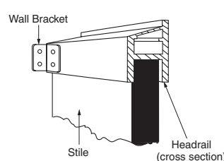
Stile Headrail (cross section)
